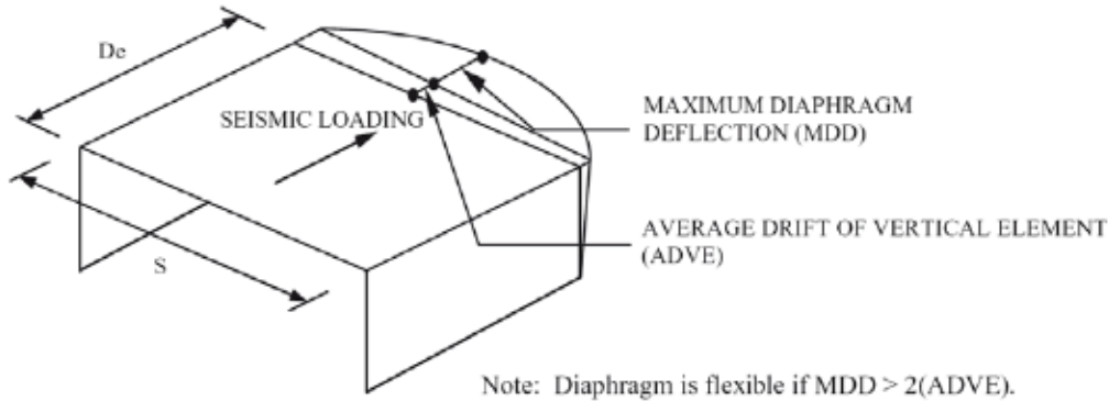
Figure 1 Flexible diaphragm
